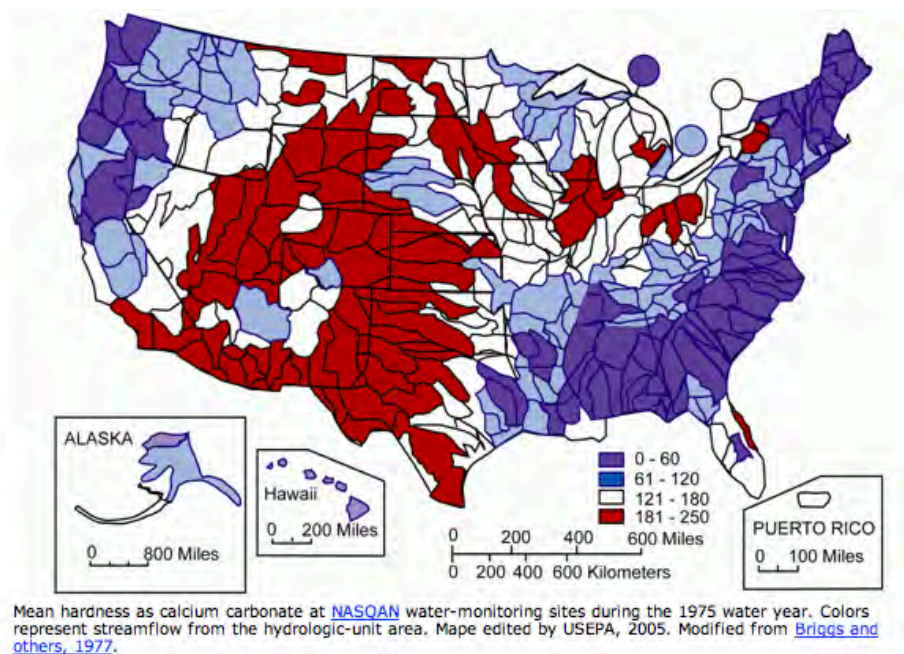
Figure 15. Average Water Hardness Across the United States as Calcium Carbonate (in milligrams per liter).
